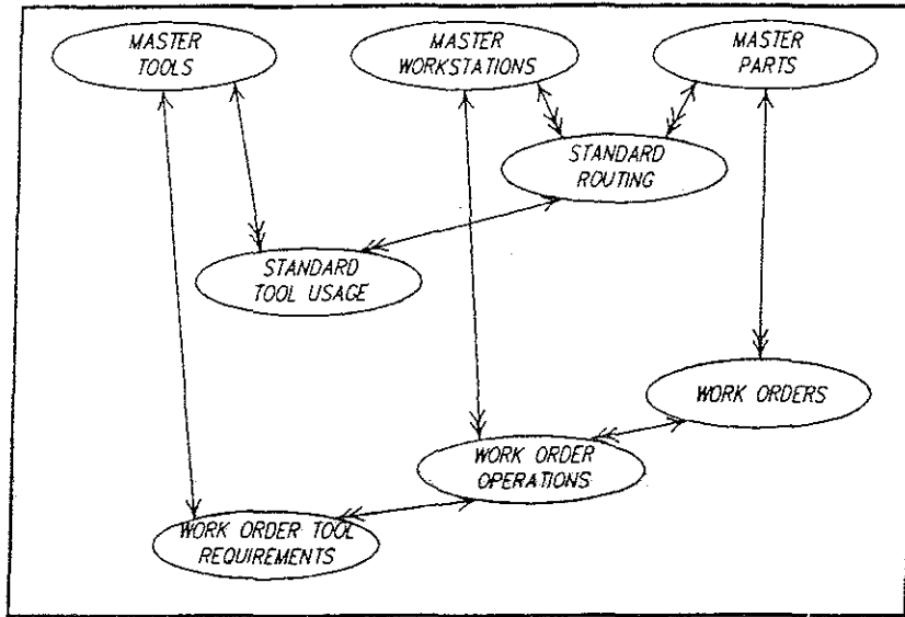
FIGURE 6. ENTITY RELATIONSHIP MODEL
