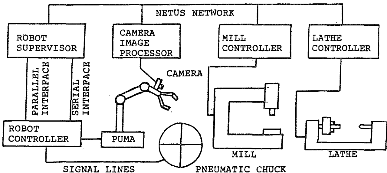
FIGURE 3: THE KNOWLEDGE BASED FMS LAYOUT
