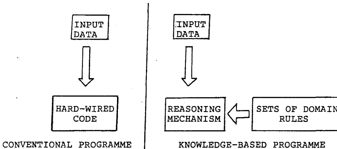
FIGURE 1 : STRUCTURES OF CONVENTIONAL AND KNOWLEDGE BASED PROGRAMMES (Swift 1983)
