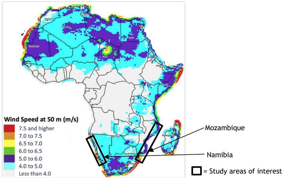
Figure 5: Elevated wind speeds across the African continent (Source: Mukasa [13]) (see online version for colour)
