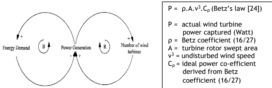
Figure 9: Betz's law and power generation feedback loops (Source: Goh et al. [24])
