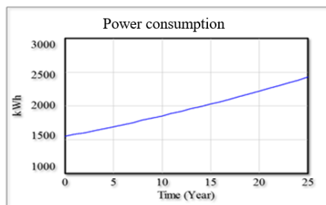
Figure 10c: Energy growth over turbine lifetime for Namibia (Source: Authors)
