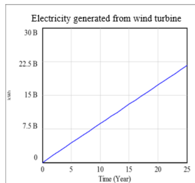
Figure 13b: Turbine electricity generation for Mozambique (Source: Authors)
