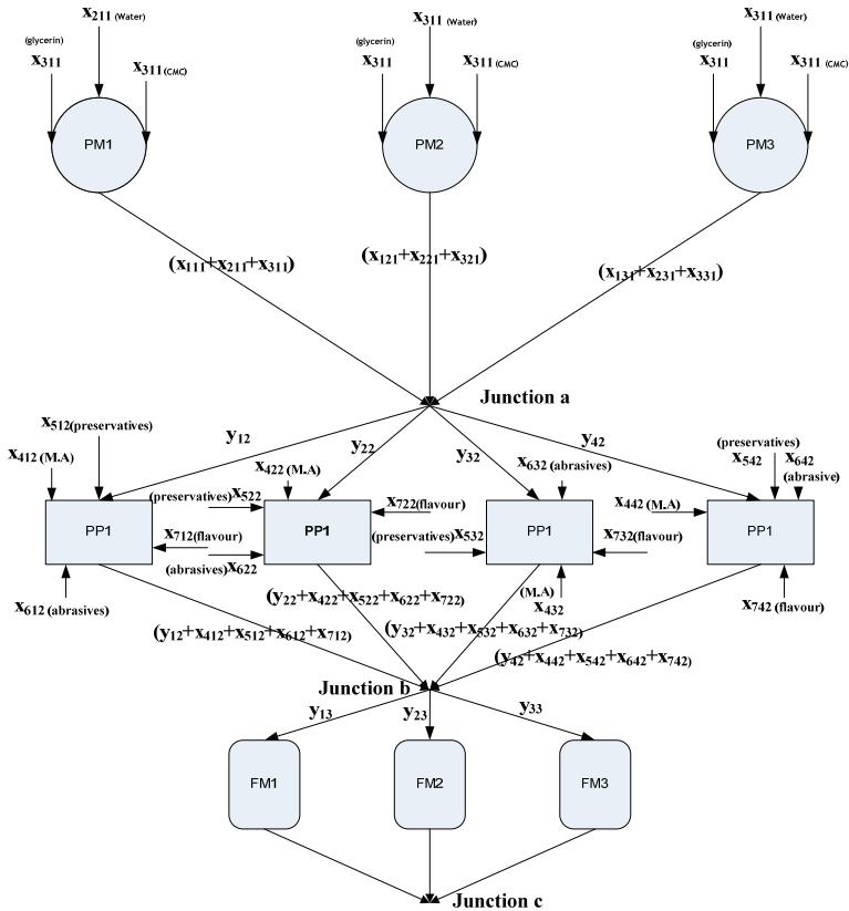
Figure 1: Process flow diagram for toothpaste production
